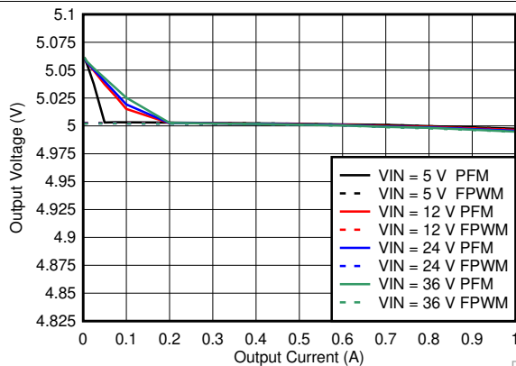
图 78. Line and Load Regulation for V_{OUT} = 5\text{ V}
