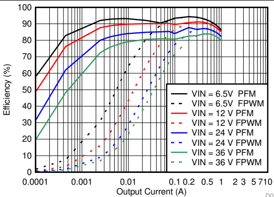
MODE = Low for Auto PFM Mode MODE = High for FPWM Mode 5-V Fixed Output
