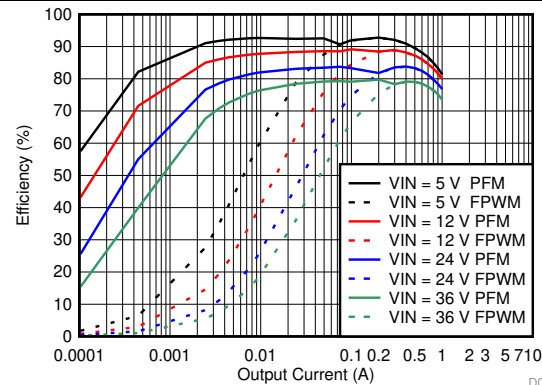
MODE = Low for Auto PFM Mode MODE = High for FPWM Mode 3.3-V Fixed Output
