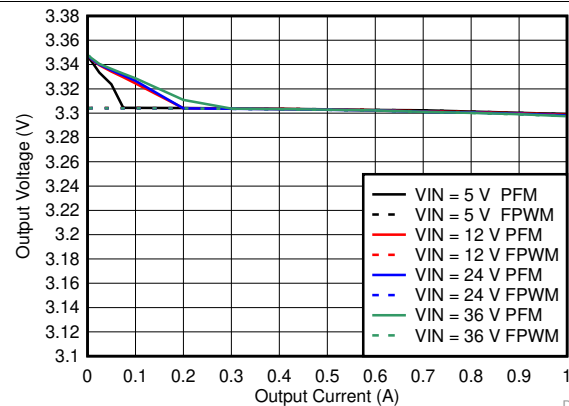
图 79. Line and Load Regulation for V_{OUT} = 3.3\text{ V}
