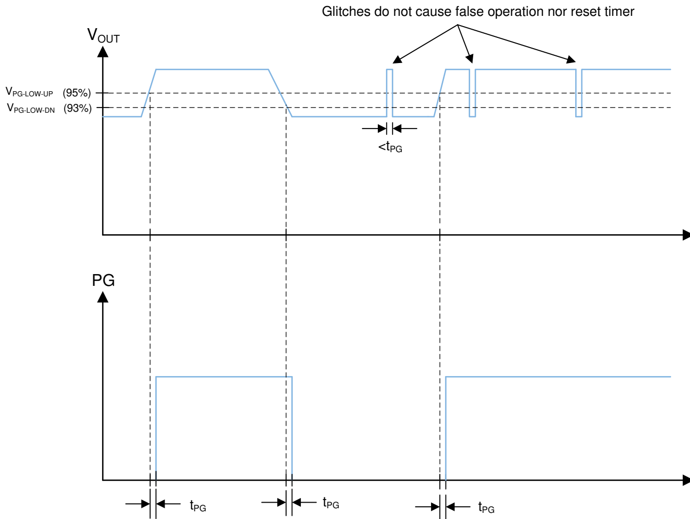
图 9. Power-Good-Timing Behavior
