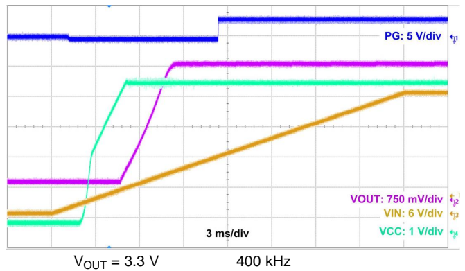
图 33. Start-Up Waveform
