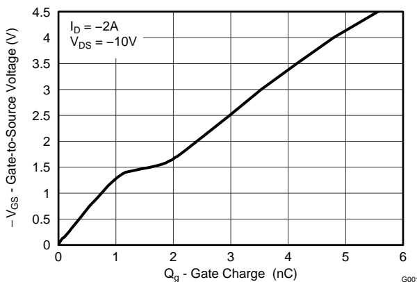
栅极电荷
