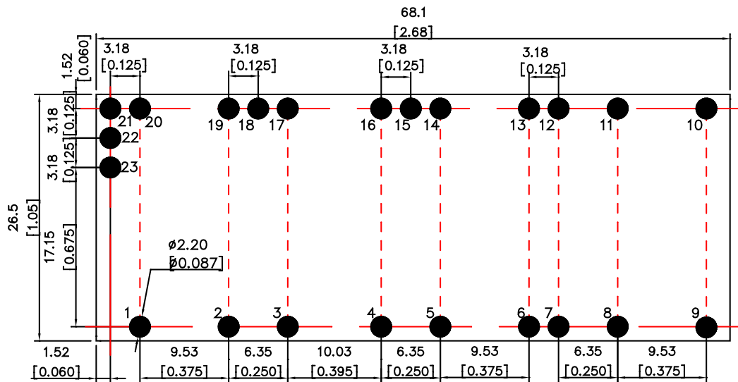
Component-side footprint
