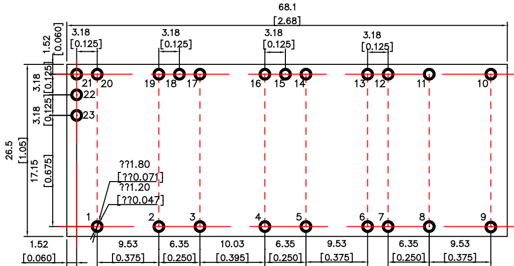
Component-side footprint
