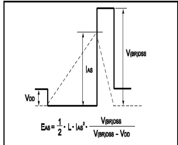
Fig.12 Avalanche Waveform
