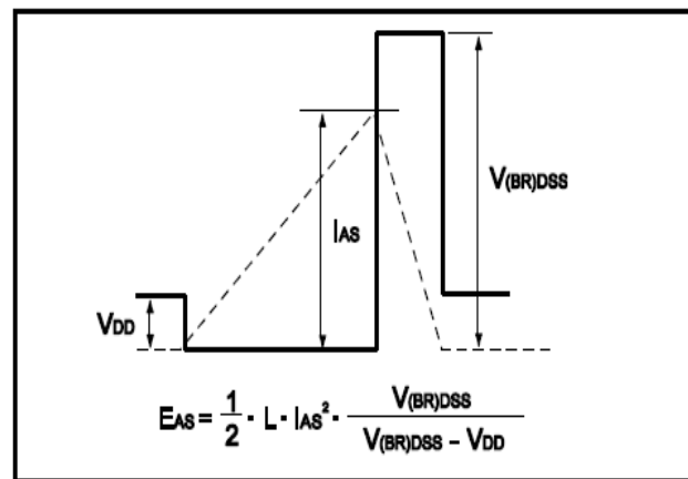
Fig.6 Avalanche Waveform
