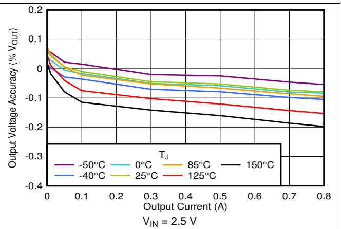
图 2. V_{OUT} Accuracy vs I_{OUT}
