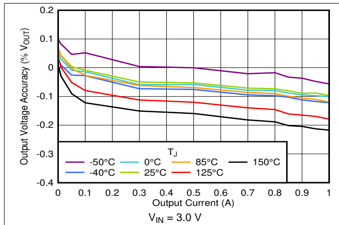
图 1. V_{OUT} Accuracy vs I_{OUT}
