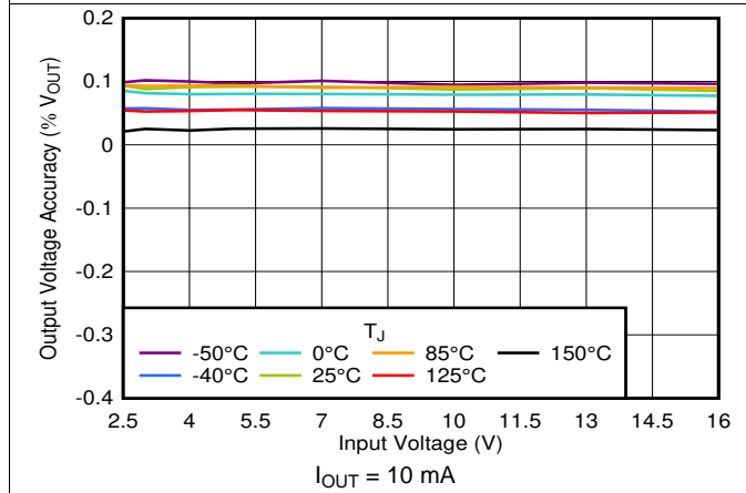
图 3. V_{OUT} Accuracy vs V_{IN}
