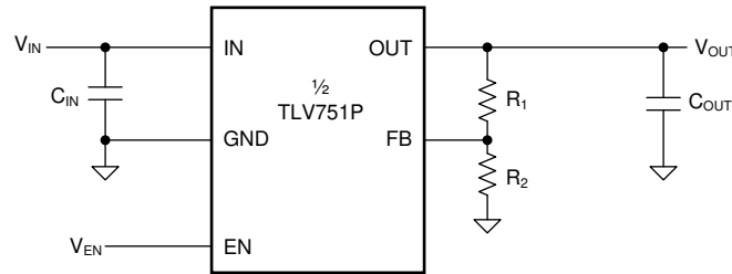
图 42. TLV751 Typical Application
