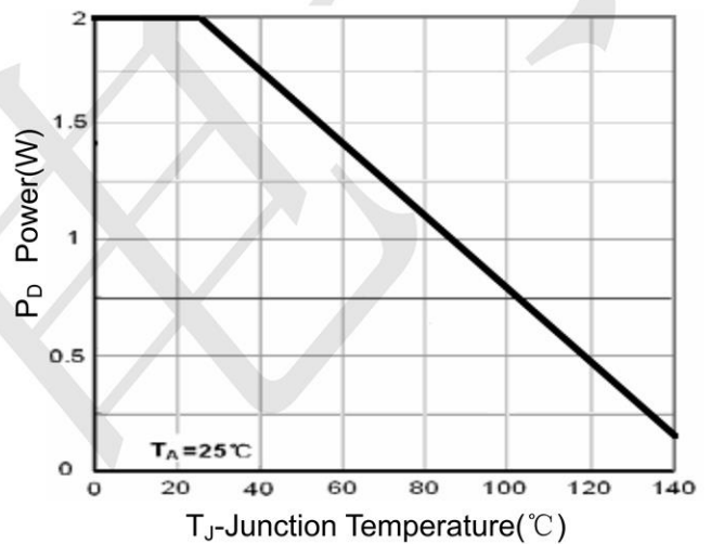
Figure 10 Power Dissipation
