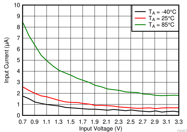
TPS610986 MODE = Low V (MAIN) = 3.3 V
