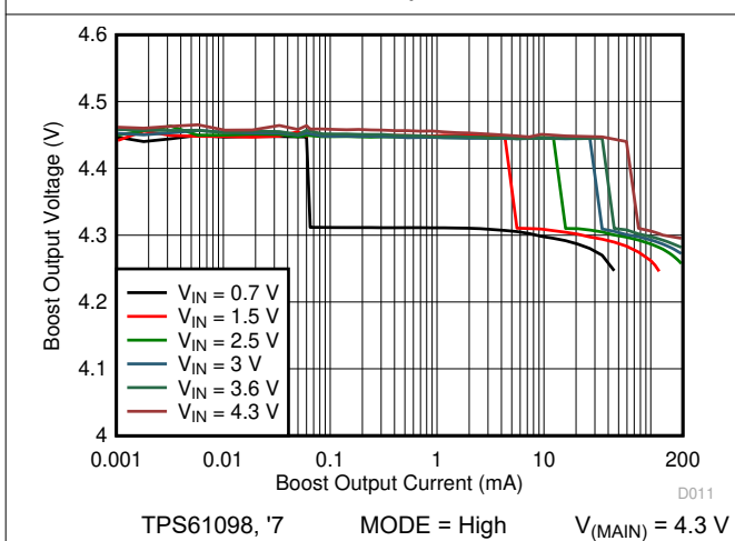
图 7-29. Boost Load Regulation (Active Mode)
