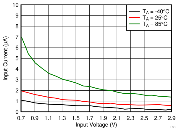
TPS610985 MODE = Low V (MAIN) = 3 V
