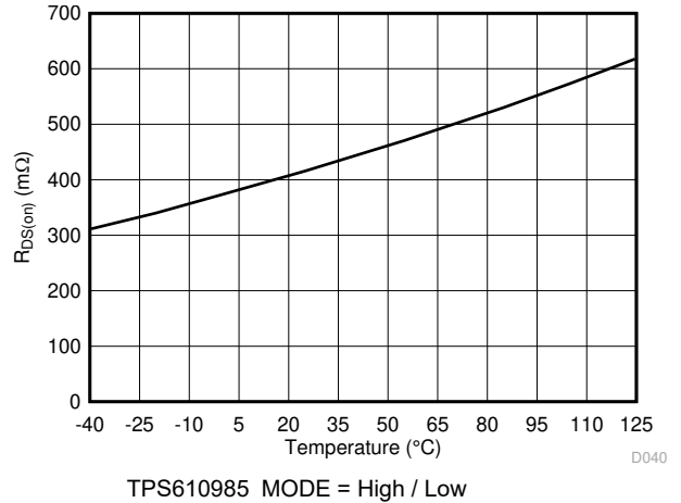
图 7-14. Low Side Switch On Resistance vs Temperature
