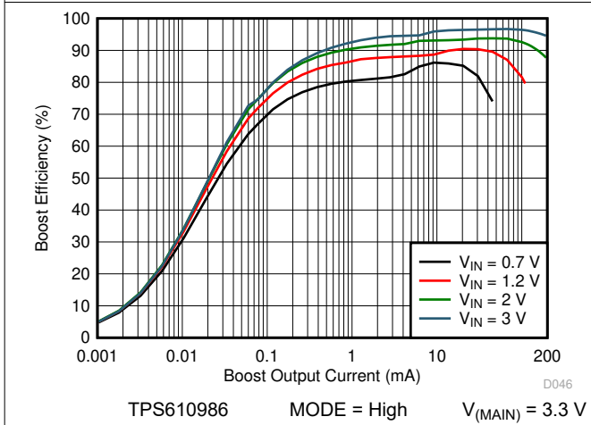
图 7-27. Boost Efficiency vs Output Current (Active Mode)
