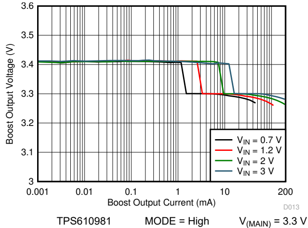
图 7-31. Boost Load Regulation (Active Mode)
