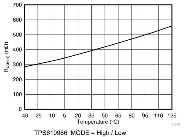
图 7-16. Low Side Switch on Resistance vs Temperature
