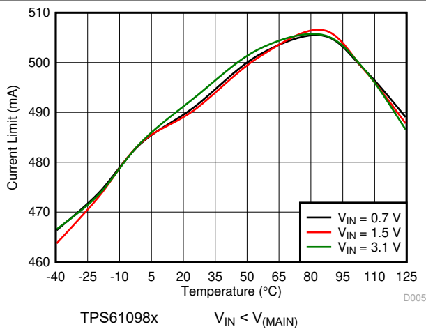
图 7-17. Current Limit vs Temperature
