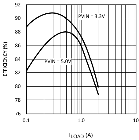
Figure 1. Efficiency vs I_{Load} V_{OUT} = 1.5\text{ V}
