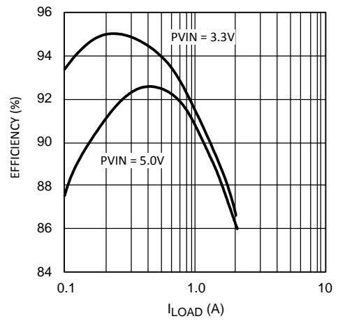
Figure 2. Efficiency vs I_{Load} V_{OUT} = 2.5\text{ V}
