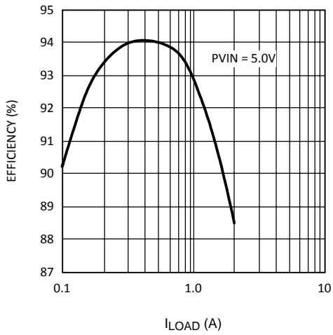
Figure 3. Efficiency vs I_{Load} V_{OUT} = 3.3\text{ V}
