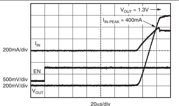
V_{IN} = 1.8\text{ V} V_{OUT} = 1.3\text{ V} V_{BIAS} = 2.7\text{ V} I_{OUT} = 350\text{ mA}
