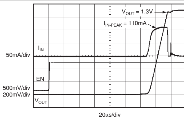
V_{IN} = 1.8\text{ V} V_{OUT} = 1.3\text{ V} V_{BIAS} = 2.7\text{ V} I_{OUT} = 0\text{ mA}
