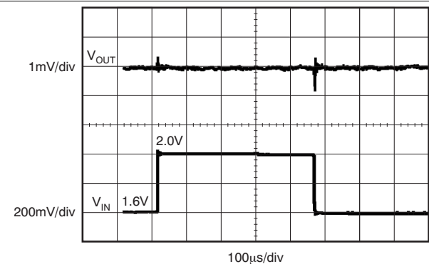
V_{IN} = 1.6\text{ to }2\text{ V} V_{OUT} = 1.3\text{ V} V_{BIAS} = 2.7\text{ V} V_{IN} Slew Rate = 1\text{ V}/\mu\text{s} I_{OUT} = 350\text{ mA}
