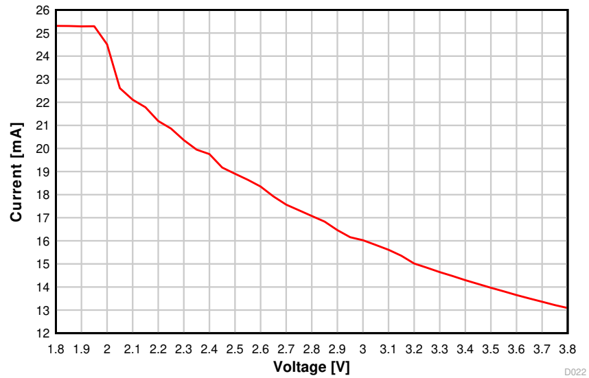
图 8-15. TX Current vs. Supply Voltage (VDD5) (50 kbps, 868.3 MHz)
