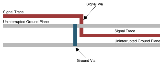
图 11-9. Ground Via Location (Side View)
