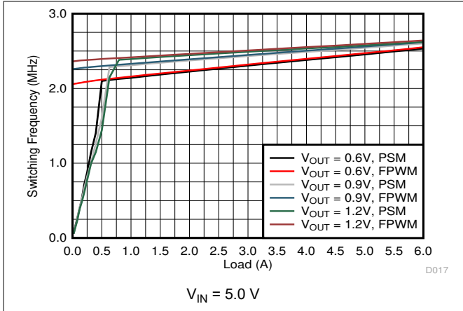
图 9-8. Switching Frequency
