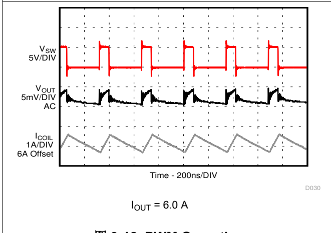
图 9-12. PWM Operation
