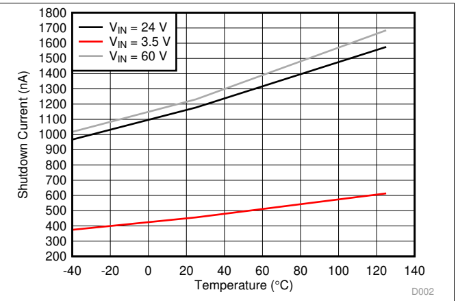
图 2. Shutdown Quiescent Current
