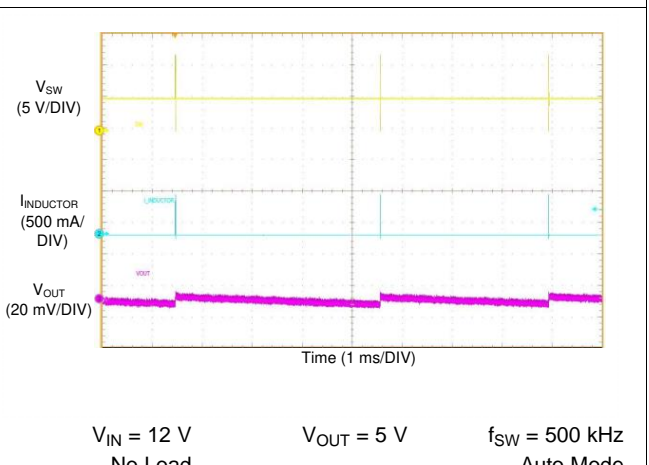
图 58. LM76003-Q1 Switching Waveform and Output Ripple
