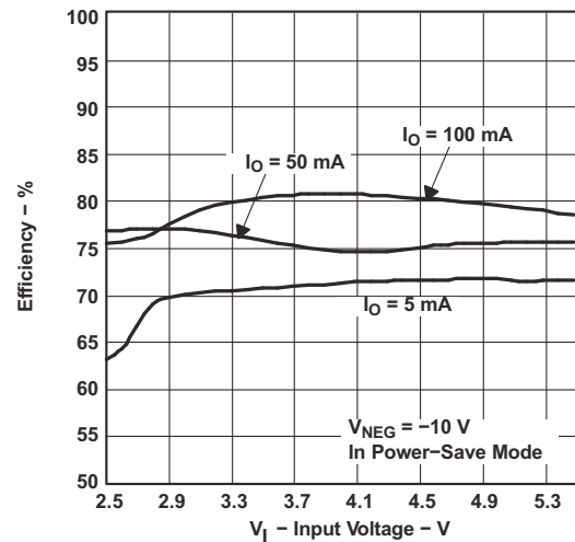
图 8-19. TPS65130 Efficiency vs Input Voltage
