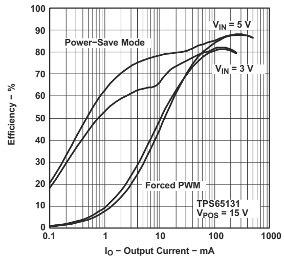
图 8-7. TPS65131 Efficiency vs Output Current
