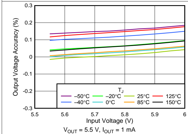
图 3. 5.5-V Line Regulation vs V_{IN}
