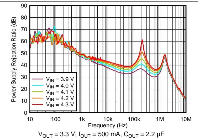
图 26. PSRR vs Frequency and V_{IN}
