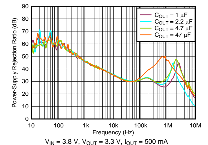
图 30. PSRR vs Frequency and C_{OUT}
