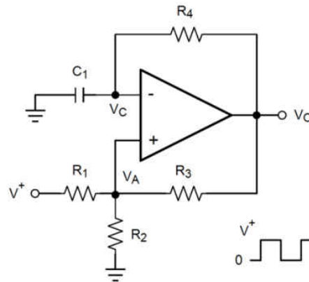
图 8-7. Square-Wave Oscillator
