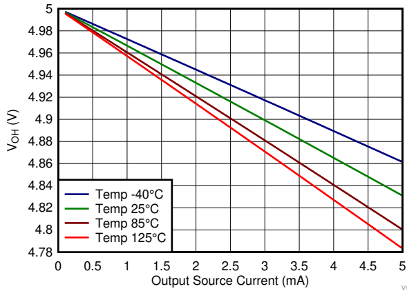
图 6-15. Output Voltage High vs Output Source Current
