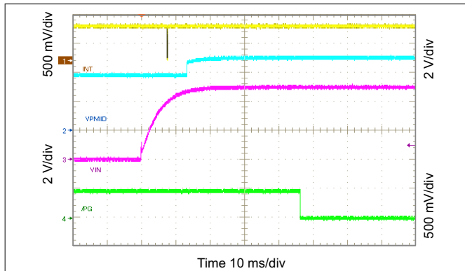
图 10-57. Show \overline{PG} and \overline{INT} Timing ( V_{IN} Insertion)
