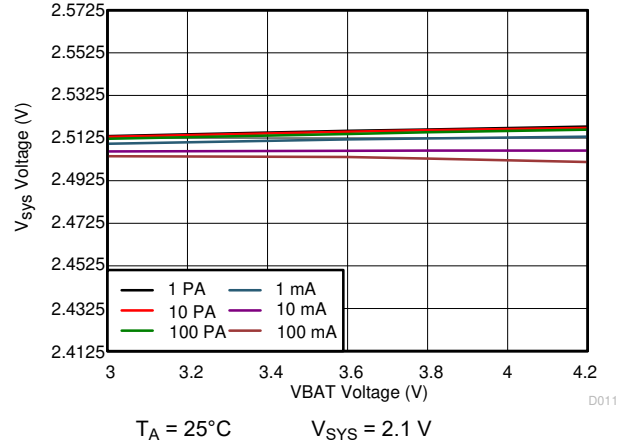
图 10-21. 2.1 V sys Line Regulation
