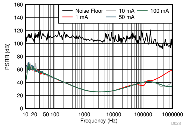
图 8-14. LS/LDO PSRR vs Frequency
