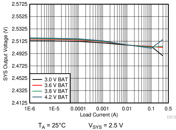
图 10-16. 2.5 V sys Load Regulation
