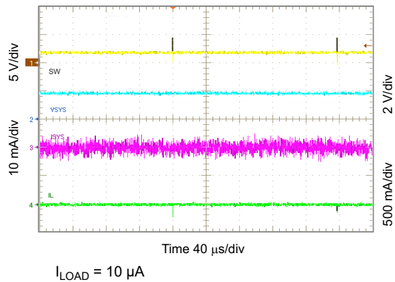
图 10-24. Light Load Operation Showing SW
