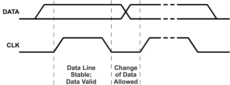
图 9-8. Bit Transfer on the Serial Interface
