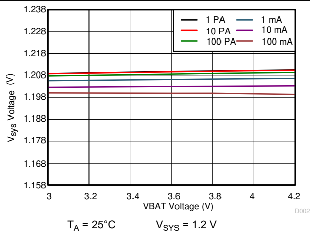
图 10-18. 1.2 V sys Line Regulation
