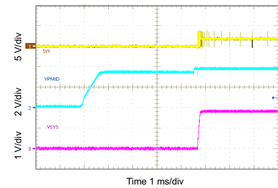
图 10-41. Startup Showing SS on SYS in PWM Mode
