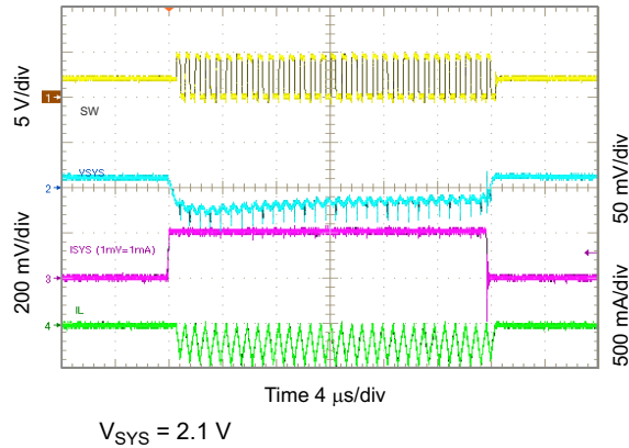
图 10-38. 2.1 V SYS Load Transient, 0 to 200 mA
