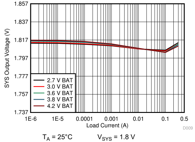
图 10-15. 1.8 V sys Load Regulation
