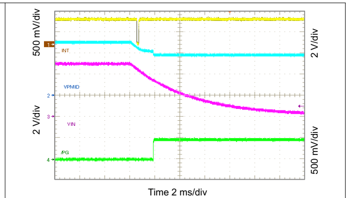
图 10-58. Show \overline{PG} and \overline{INT} Timing ( V_{IN} Removal)
