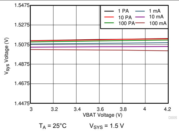
图 10-19. 1.5 V sys Line Regulation
