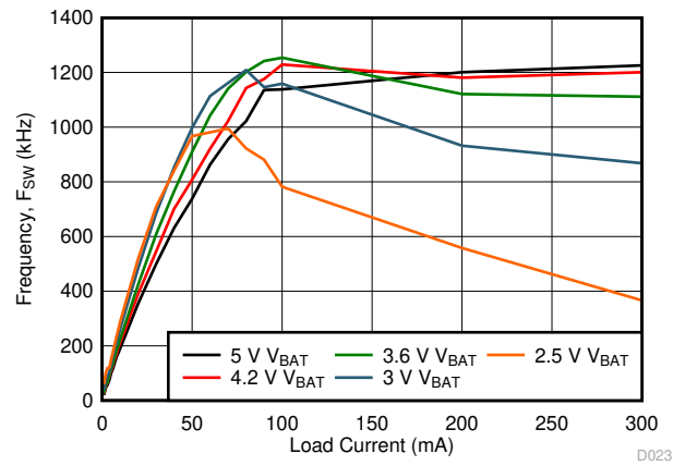
图 10-23. 1.8 V sys Switching Frequency vs Load Current
