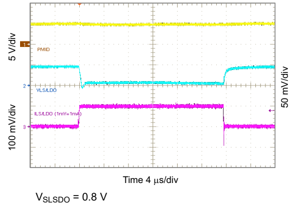
图 10-50. 0.8 V_{LSLDO} Load Transient, 0 to 100 mA
