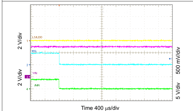
图 10-59. \overline{PG} Functions as Shifted \overline{MR} Output
