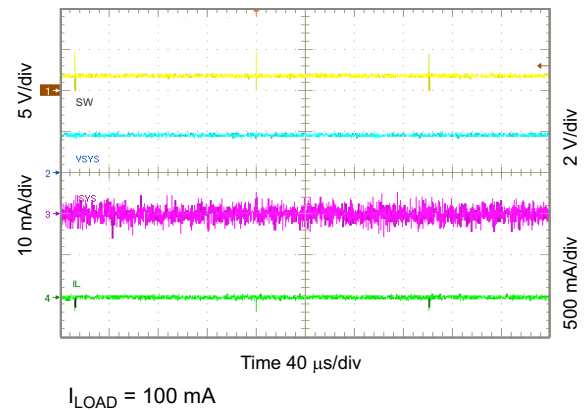
图 10-25. Light Load Operation Showing SW
