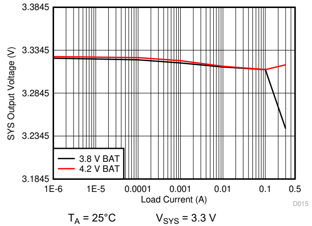
图 10-17. 3.3 V sys Load Regulation
