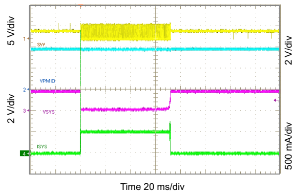
图 10-42. Short Circuit and Recovery for SYS
