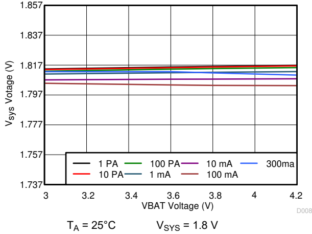
图 10-20. 1.8 V sys Line Regulation
