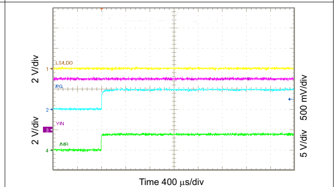
图 10-60. \overline{PG} Functions as Shifted \overline{MR} Output
