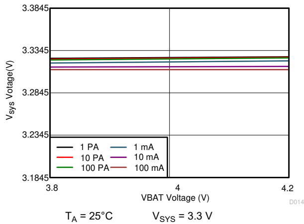
图 10-22. 3.3 V sys Line Regulation
