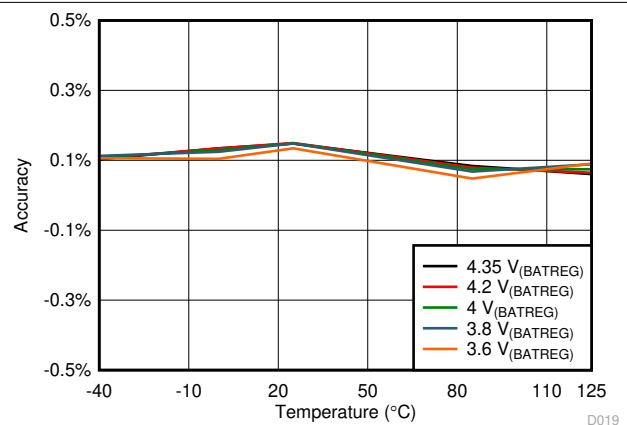
图 8-8. V BATREG Accuracy vs Temperature
