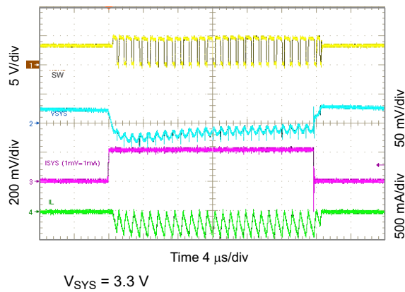
图 10-40. 3.3 V SYS Load Transient, 0 to 200 mA
