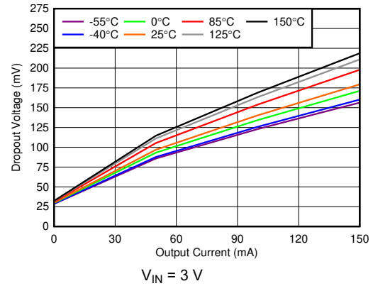
图 6-8. Dropout Voltage ( V_{DO} ) vs I_{OUT}
