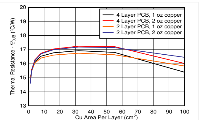
图 8-3. \psi_{JB} vs Copper Area 2s2p DCY Package
