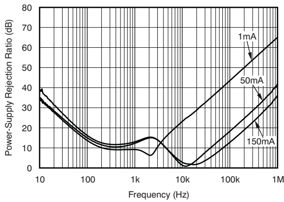
Figure 13. TPS78330 Ripple Rejection vs Frequency
