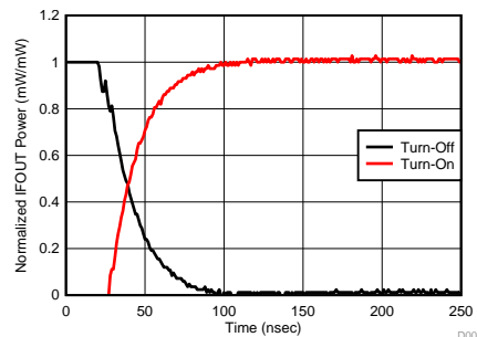
Figure 74. Device power down turn-on and turn-off time
