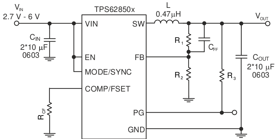
图 10-1. Typical Application
