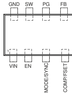
图 6-1. 8-Pin SOT583 DRL Package (Top View)
