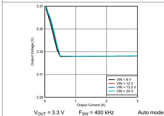
图 9-12. LM61430-Q1 Load and Line Regulation
