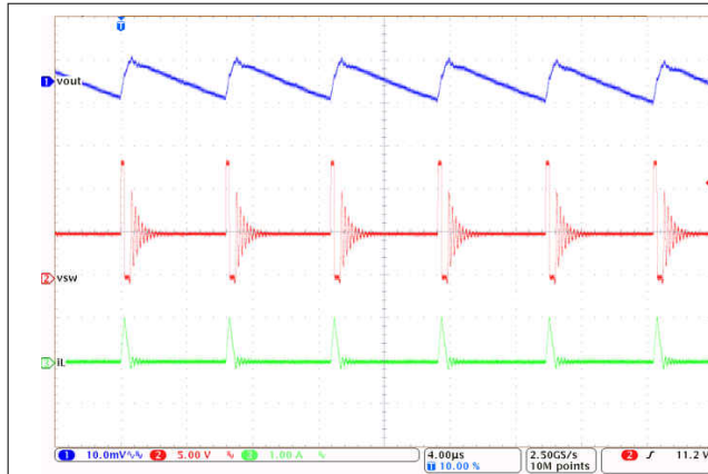
图 9-28. LM61430-Q1 Switching Waveform and V_{OUT} Ripple
