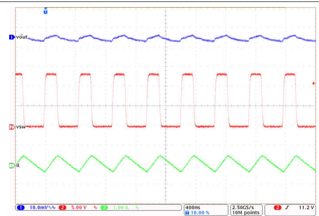
图 9-29. LM61430-Q1 Switching Waveform and V_{OUT} Ripple
