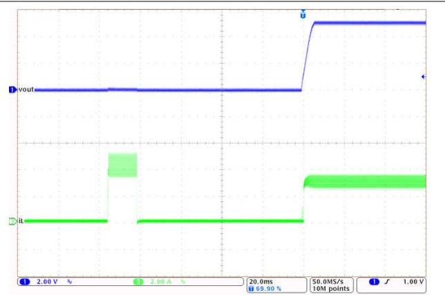
图 8-13. Short-Circuit Recovery
