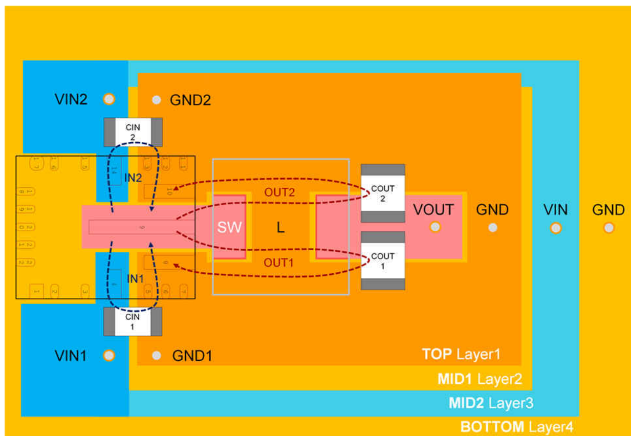
图 11-1. Layout of the Power Components and Current Flow
