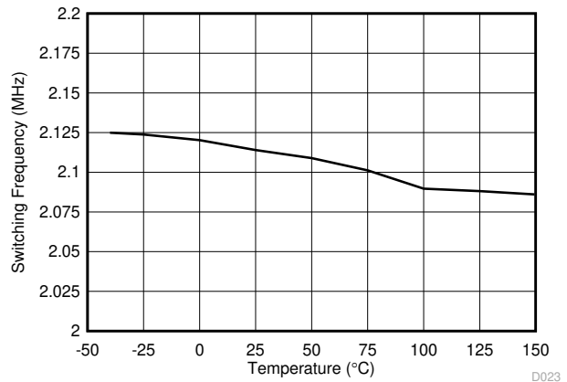
图 7-2. Switching Frequency vs Temperature
