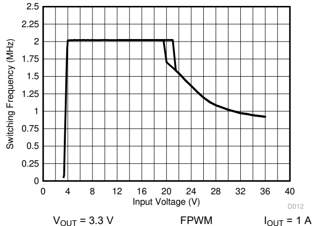
图 9-28. Switching Frequency vs Input Voltage
