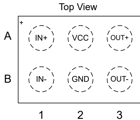
图 5-2. WCSP Package 6-Pin BGA Top View
