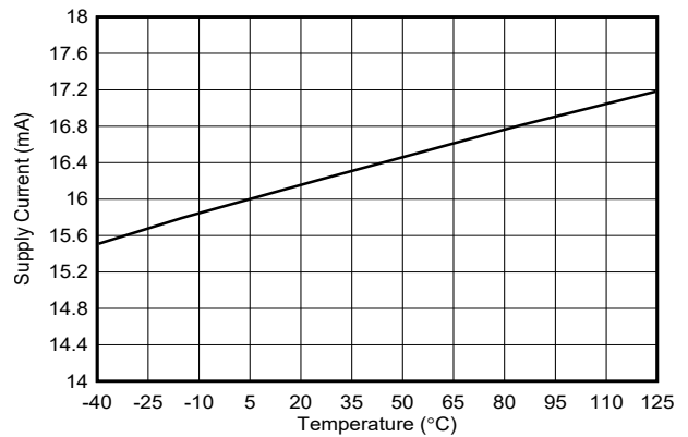
图 6-10. TLV3811 Supply Current vs. Temperature
