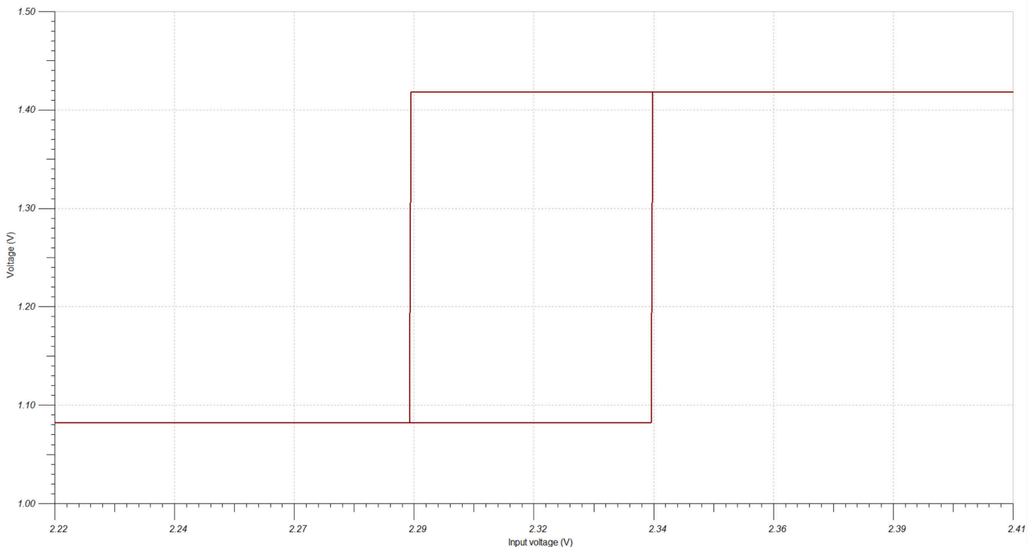
图 8-4. Hysteresis Curve for LVDS Comparator
