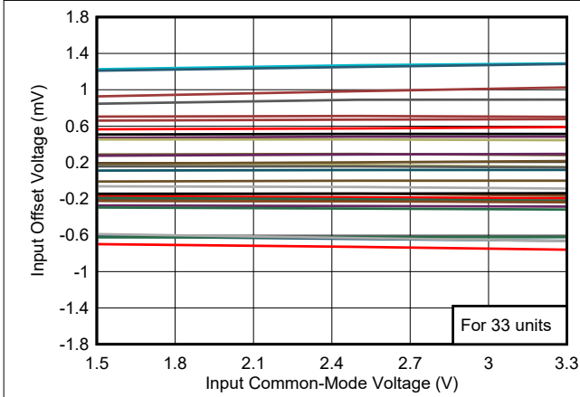
图 6-5. Offset vs. Common-Mode, 3.3 V
