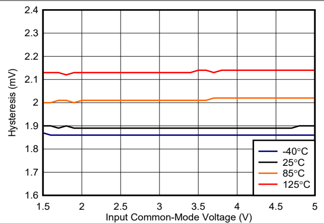
图 6-8. Hysteresis vs. Common-Mode, 5 V
