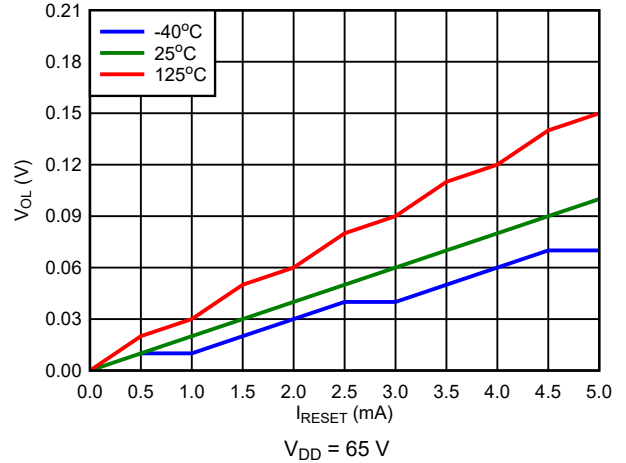
图 7-10. Open-Drain Active Low V_{OL} vs I_{RESET}
