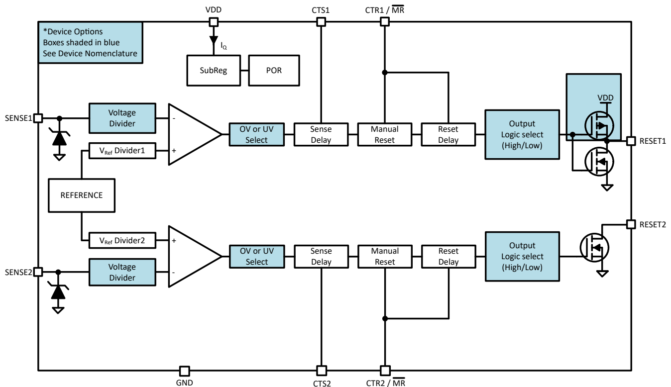
图 8-1. Functional Block Diagram 1
