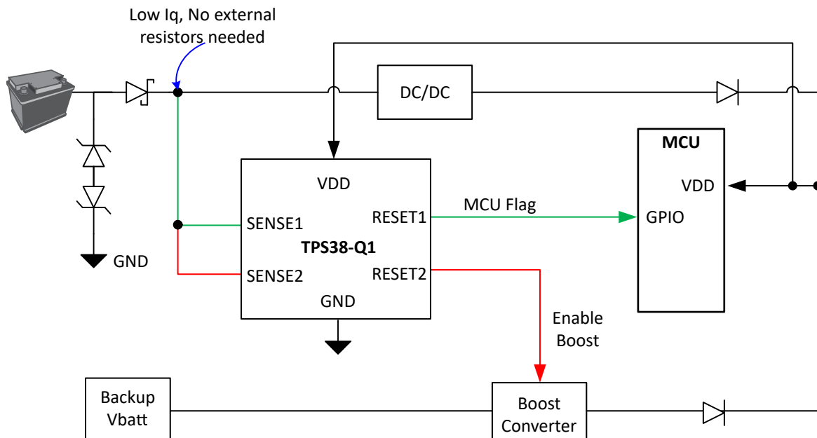
图 10-2. Fast Start Supervisor with Direct Off-Battery Monitoring
