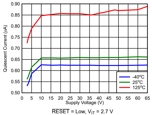
图 7-4. V_{DD} vs I_{DD} ( \overline{\text{RESET}} = \text{Low} , V_{IT} = 2.7\text{ V} )
