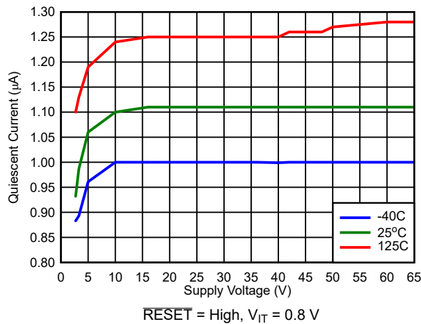
图 7-5. V_{DD} vs I_{DD} ( \overline{\text{RESET}} = \text{High} , V_{IT} = 0.8\text{ V} )
