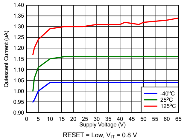
图 7-6. V_{DD} vs I_{DD} ( \overline{\text{RESET}} = \text{Low} , V_{IT} = 0.8\text{ V} )
