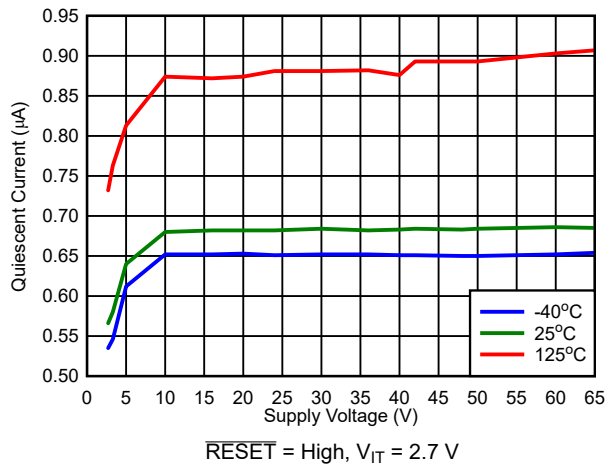
图 7-3. V_{DD} vs I_{DD} ( \overline{\text{RESET}} = \text{High} , V_{IT} = 2.7\text{ V} )
