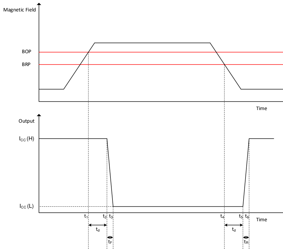
图 8-8. Propagation Delay
