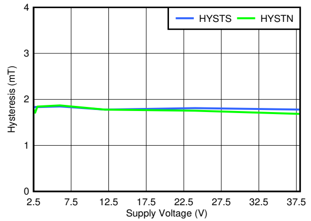
图 7-14. TMAG5123D Hysteresis vs Supply Voltage
