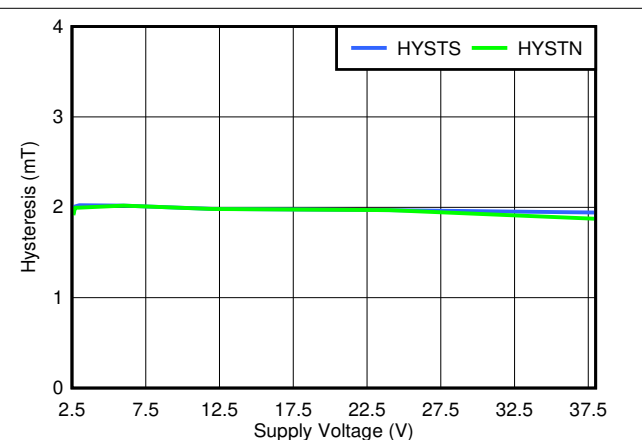
图 7-6. TMAG5123B Hysteresis vs Supply Voltage
