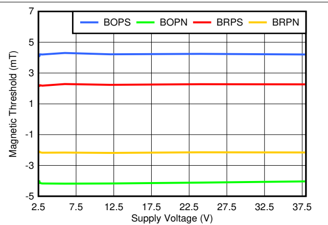
图 7-4. TMAG5123B Magnetic Thresholds vs Voltage
