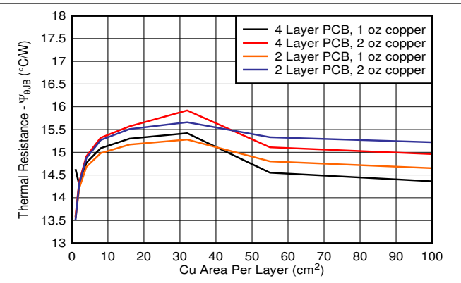
8-5. \Psi_{JB} vs Copper Area 2s2p DCY Package
