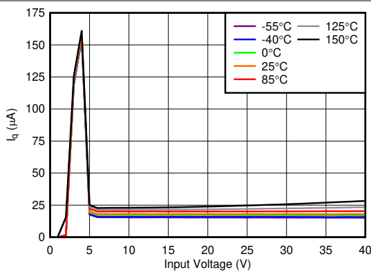
V_{OUT} = 5\ \text{V}
