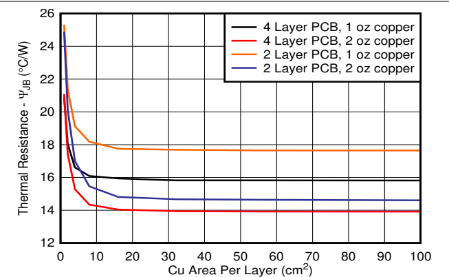
8-3. \Psi_{JB} vs Copper Area 2s2p DRB Package
