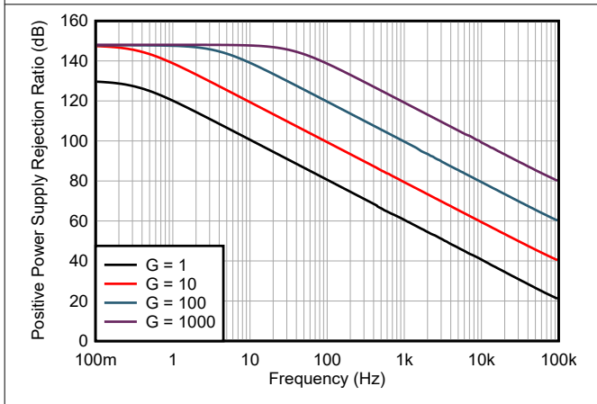
图 7-23. Positive PSRR vs Frequency (RTI)
