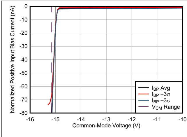
图 7-43. Positive Input Bias Current vs Common-Mode Voltage ( V_{S-} )
