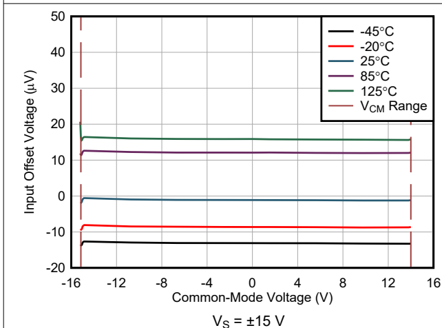
图 7-47. Offset Voltage vs Common-Mode Voltage
