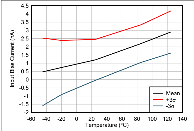
图 7-13. Input Bias Current vs Temperature
