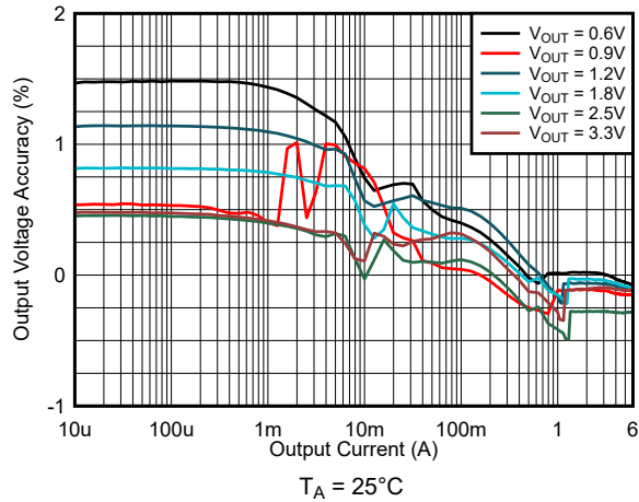
9-14. Load Regulation V_{IN} = 5.0 V and PSM
