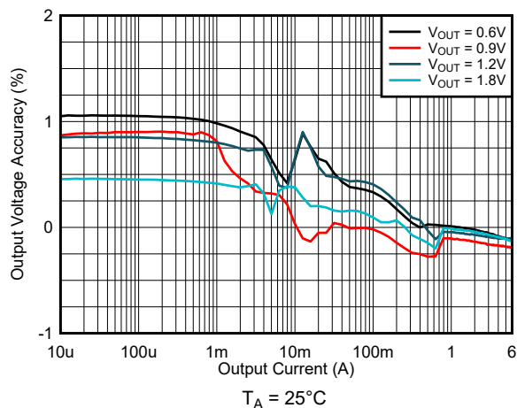
9-18. Load Regulation V_{IN} = 2.8 V and PSM
