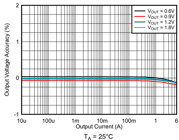
9-19. Load Regulation V_{IN} = 2.8 V and FPWM
