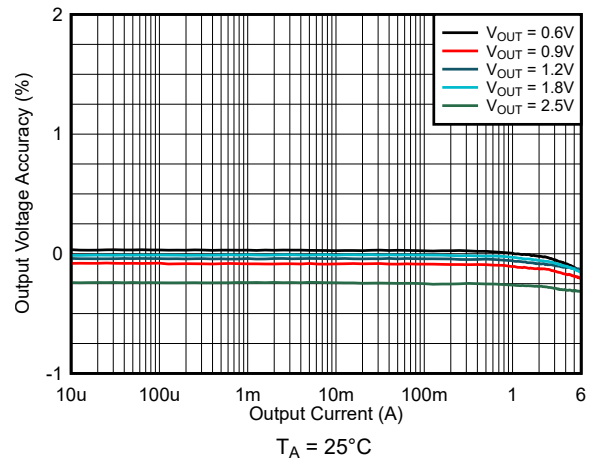
9-17. Load Regulation V_{IN} = 3.3 V and FPWM
