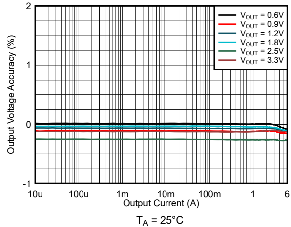
9-15. Load Regulation V_{IN} = 5.0 V and FPWM
