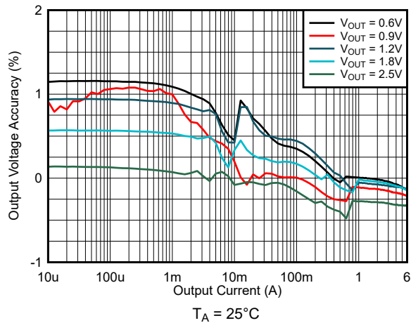
9-16. Load Regulation V_{IN} = 3.3 V and PSM
