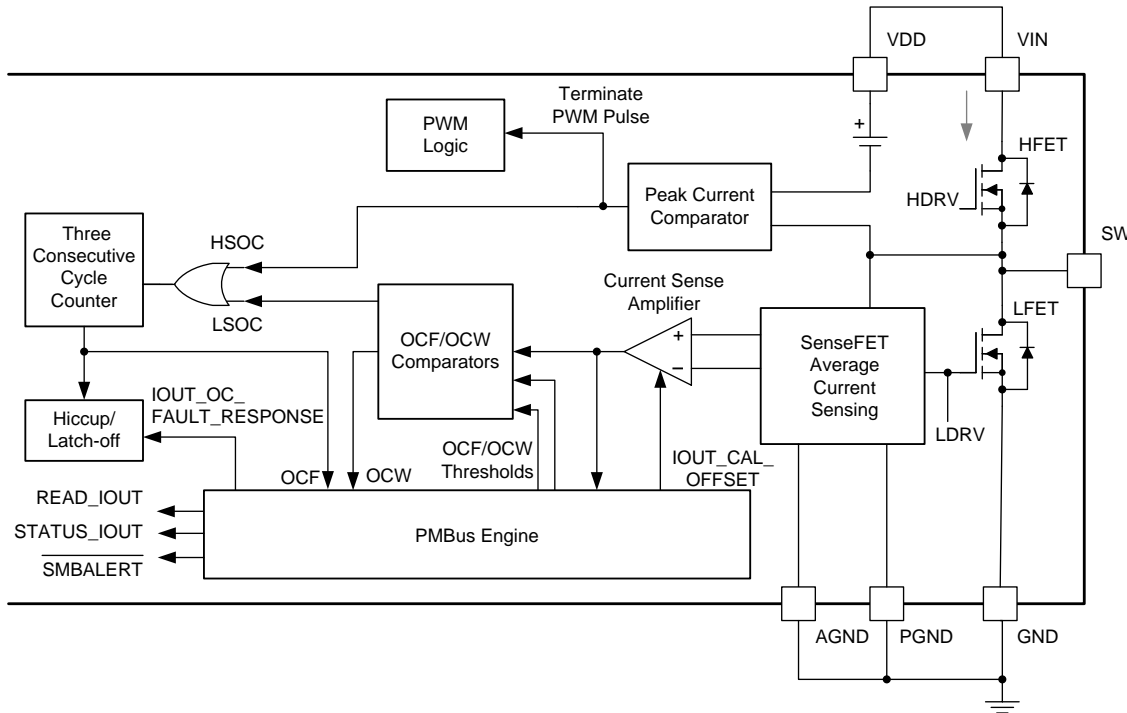
Figure 37. SenseFET Average Current Sensing and Overcurrent Protection
