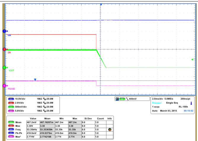
Figure 50. Shutdown from CNTL
