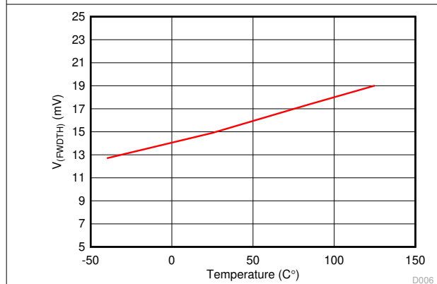
图 7-5. V_{(\text{FWDTH})} vs Temperature
