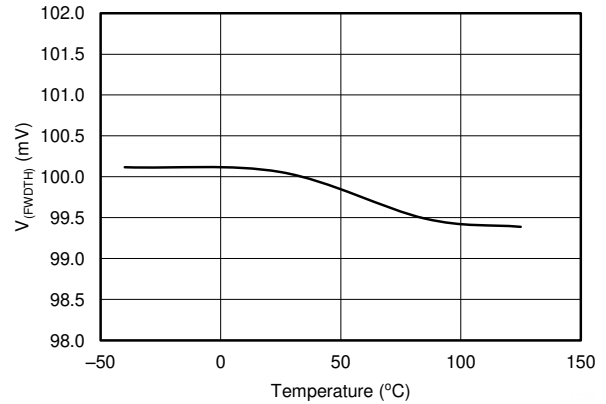
图 7-30. V (FWDTH) vs Temperature
