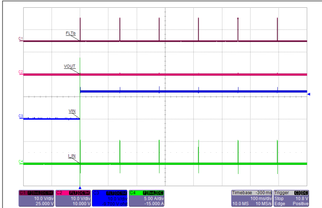
图 10-15. Hot Plug-In with Short on Output: Auto-Retry - TPS25940-Q1
