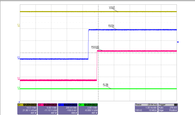
V_{(IN)} = 12\text{ V} R_L = 12\text{ }\Omega R_{(FLT)} = 100\text{ k}\Omega 图 7-38. Power Good Delay (Rising)
