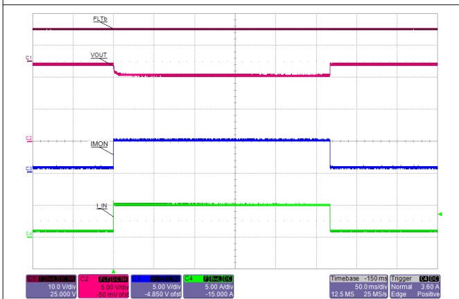
图 10-11. Over Load: Step Change in Load from 12 \Omega to 2 \Omega and Back
