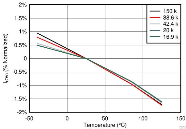
图 7-19. Current Limit (% Normalized) vs R_{(LIMIT)} Resistor
