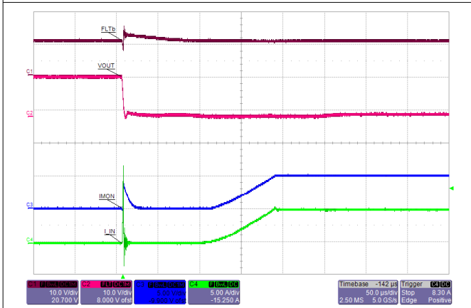
图 10-13. Hot Short: Fast Trip and Current Regulation
