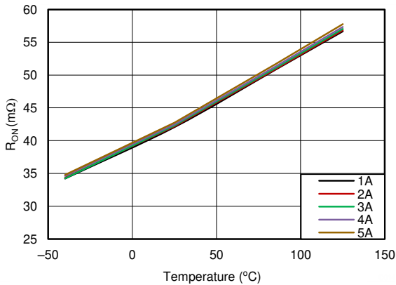
图 7-27. R ON vs Temperature Across Load Current
