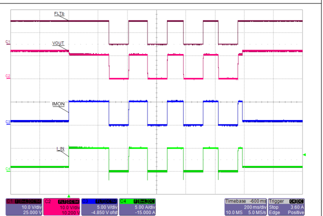
图 10-12. Overload Condition: Auto Retry and Recovery - TPS25940-Q1
