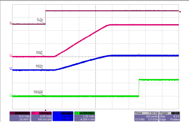
图 10-16. Power Good Response During Turn-ON
