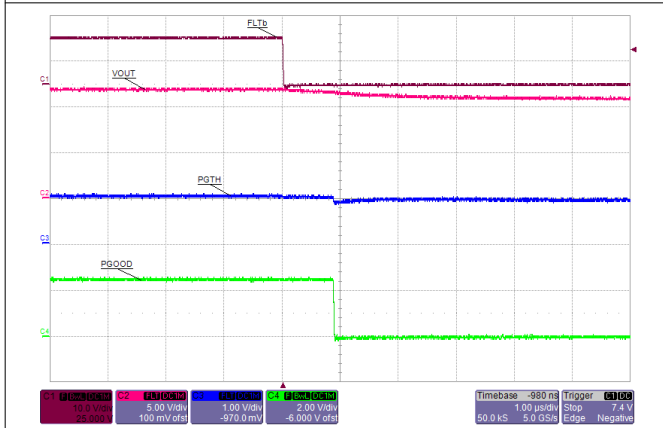
图 10-17. Power Good Response During Turn-OFF
