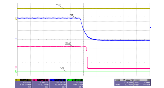
V_{(IN)} = 12\text{ V} R_L = 12\text{ }\Omega R_{(FLT)} = 100\text{ k}\Omega 图 7-39. Power Good Delay (Falling)
