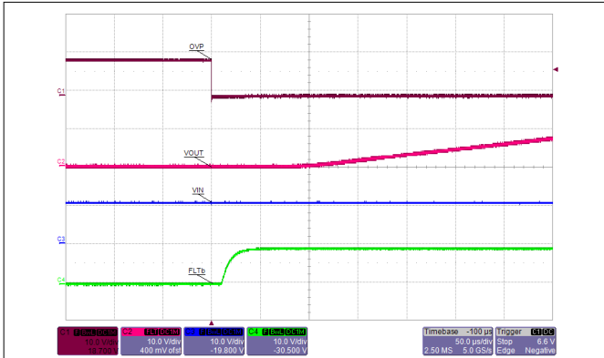
V_{(IN)} = 12\text{ V} R_L = 12\text{ }\Omega R_{(FLT)} = 100\text{ k}\Omega 图 7-37. OVP Turn ON Delay: OVP ↓ to Output Ramp ↑
