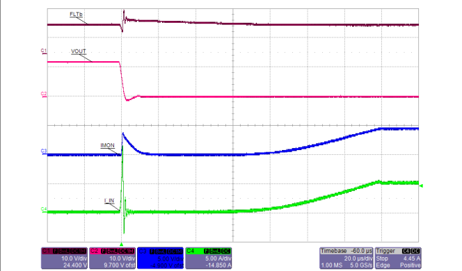
R_{(FLT)} = 100\text{ k}\Omega R_{(IMON)} = 16.9\text{ k}\Omega R_{(ILIM)} = 17.8\text{ k}\Omega 图 7-40. Hot-Short: Fast Trip Response and Current Regulation
