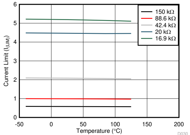
图 7-18. Current Limit vs Temperature Across R_{(ILIM)}
