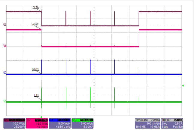
图 10-14. Hot Short: Auto-Retry and Recovery from Short Circuit - TPS25940-Q1
