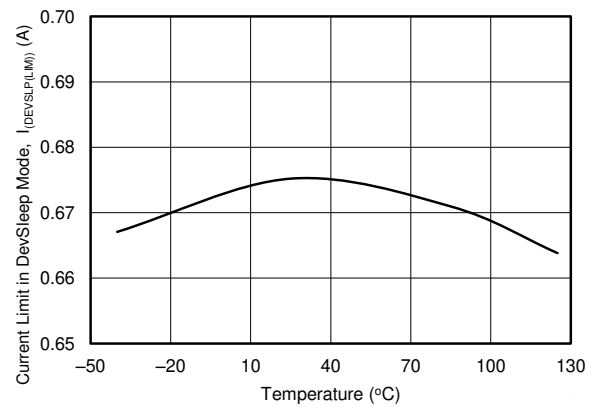
图 7-22. Current Limit in DevSleep Mode vs Temperature
