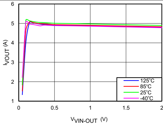
Figure 13. I_{VOUT} vs V_{VIN-OUT}
