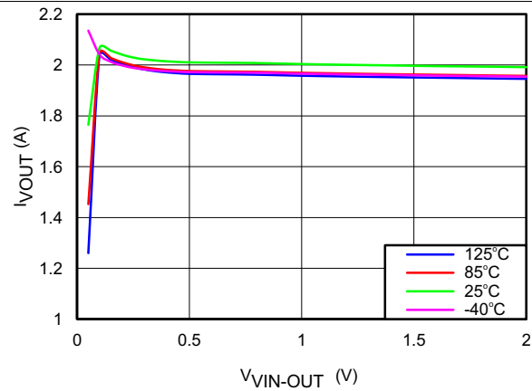
Figure 14. I_{VOUT} vs V_{VIN-OUT}
