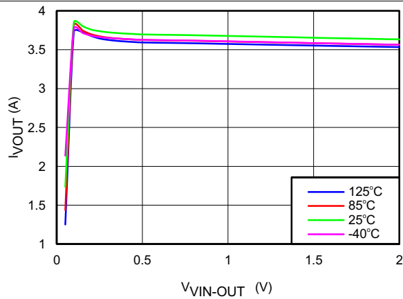
Figure 13. I_{VOUT} vs V_{VIN-OUT}
