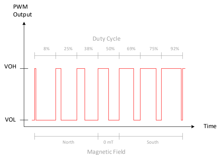
图 14. Magnetic Response
