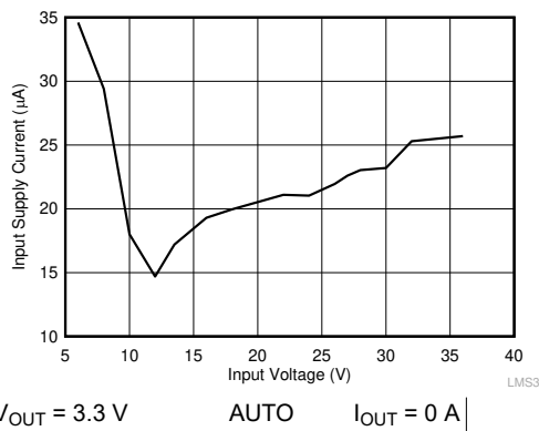
图 9-21. Input Supply Current (Includes Leakage Current of Capacitor)
