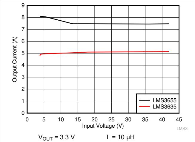
图 9-26. Output Current Level for Overcurrent Protection Trip
