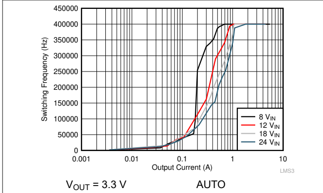
图 9-25. Switching Frequency vs Load Current
