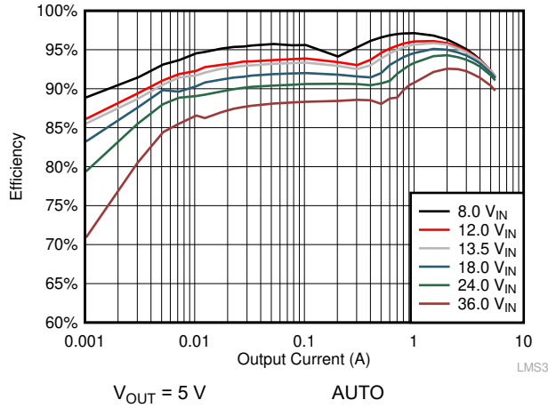
图 9-5. Efficiency
