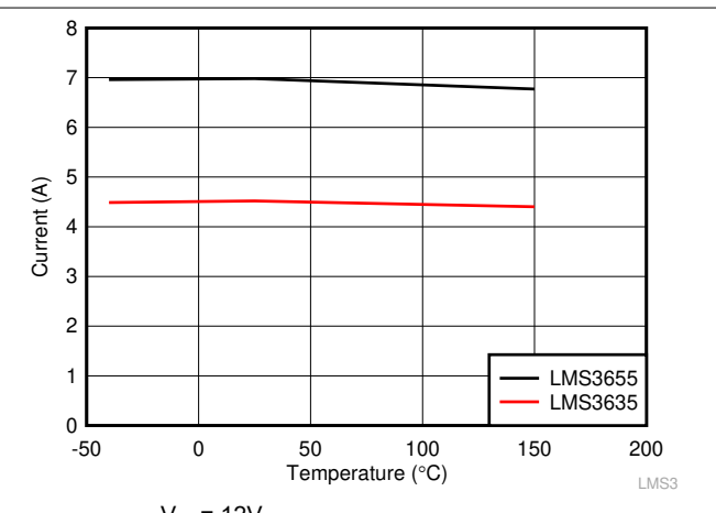
图 7-4. Low-Side/Valley Current Limit for LMS36x5-Q1
