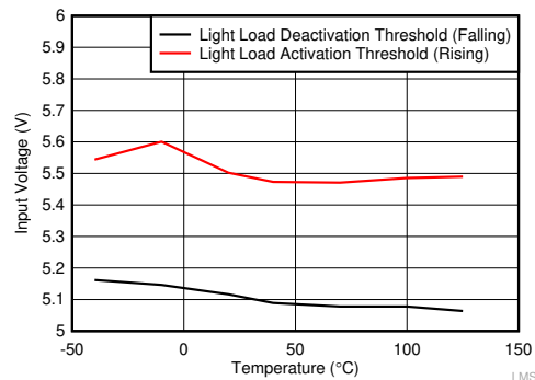
图 8-9. Input Voltage for Mode Change — 5-V Output, 10- \mu H Inductor
