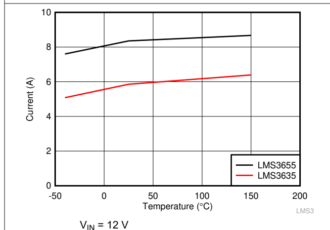
图 7-3. High-Side/Peak Current Limit for LMS36x5-Q1
