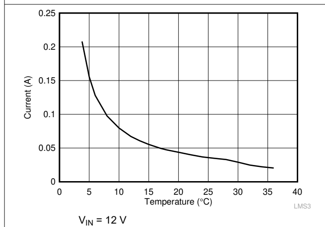
图 7-5. Short Circuit Average Input Current for LMS3635-Q1
