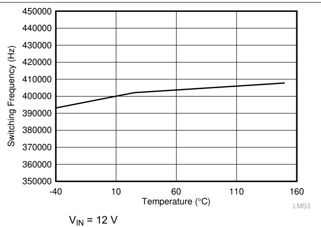
图 7-2. Switching Frequency vs Temperature
