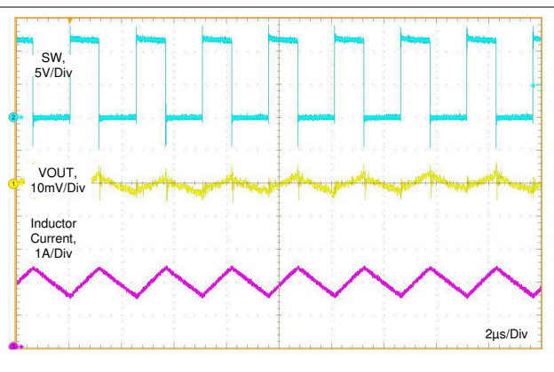
图 8-8. Typical PWM Switching Waveforms V_{IN} = 12 V, V_{OUT} = 5 V, I_{OUT} = 2 A, f_S = 400 kHz
