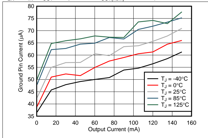
图 7. Ground Pin Current vs I_{OUT} and Temperature
