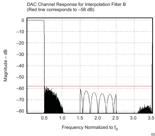
Figure 7-30. Frequency Response of Channel Interpolation Filter B
