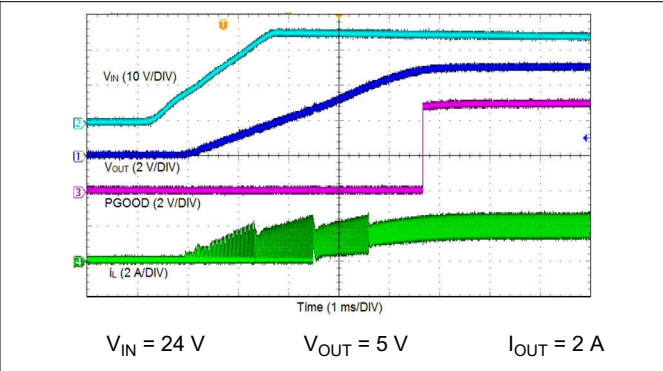
图 8-3. Start-up By VIN
