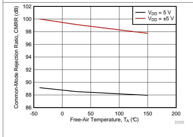
Figure 26. Common-Mode Rejection Ratio vs Free-Air Temperature
