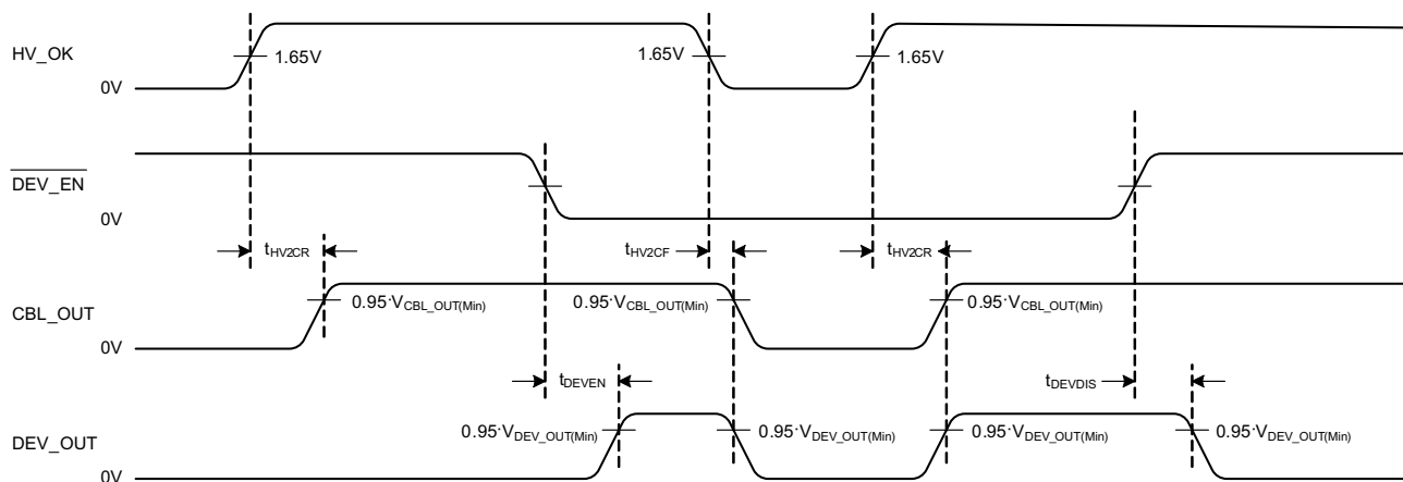
Figure 3. Timing Diagram
