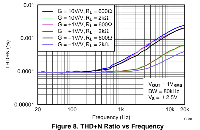
Figure 8. THD+N Ratio vs Frequency
