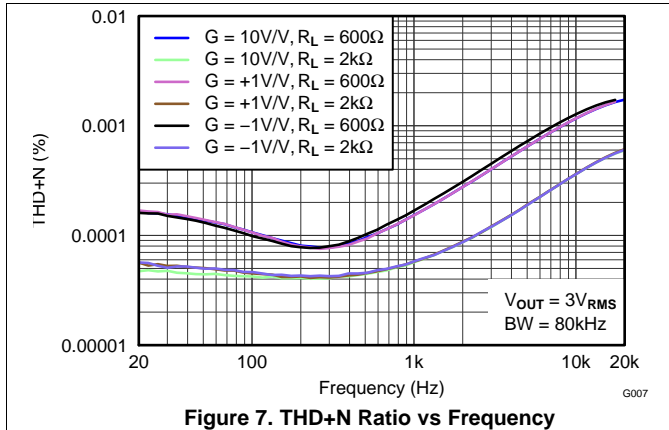
Figure 7. THD+N Ratio vs Frequency
