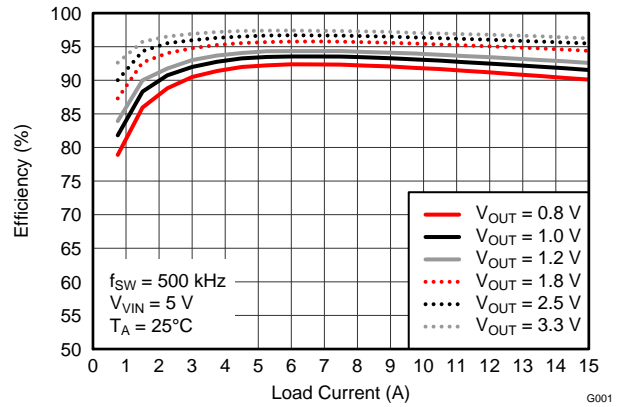
Figure 16. Efficiency vs. Load Current ( V_{VIN} = 5\text{ V} )
