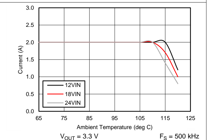
Figure 50. Derating Curve
