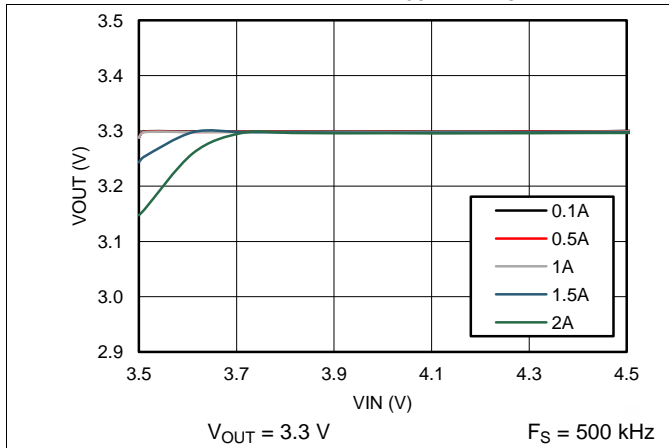
Figure 45. Dropout Voltage
