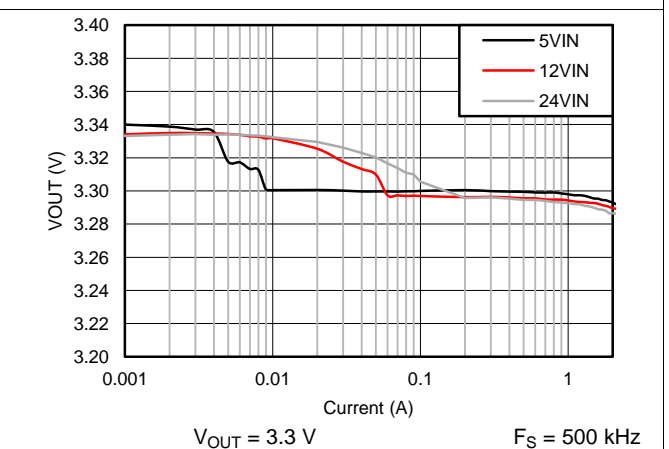
Figure 48. Regulation Curve
