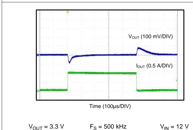
Figure 49. Load Transient
