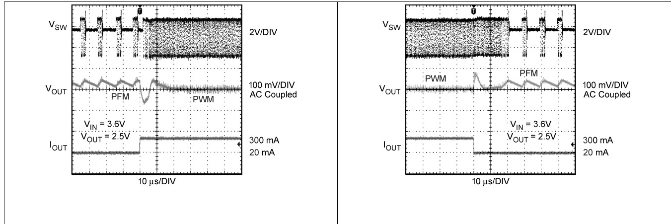
Figure 25. PFM-to-PWM Mode Change by Load Transients
