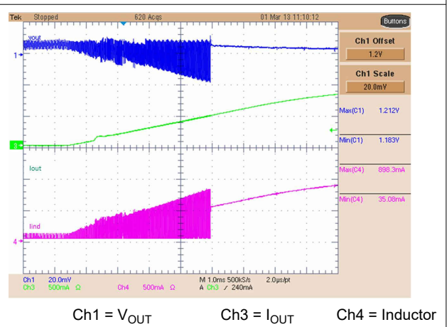
图 8-22. Buck 1 PWM to PFM Transition
