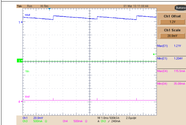
图 8-19. Buck 1 Low-Power Output, No Load
