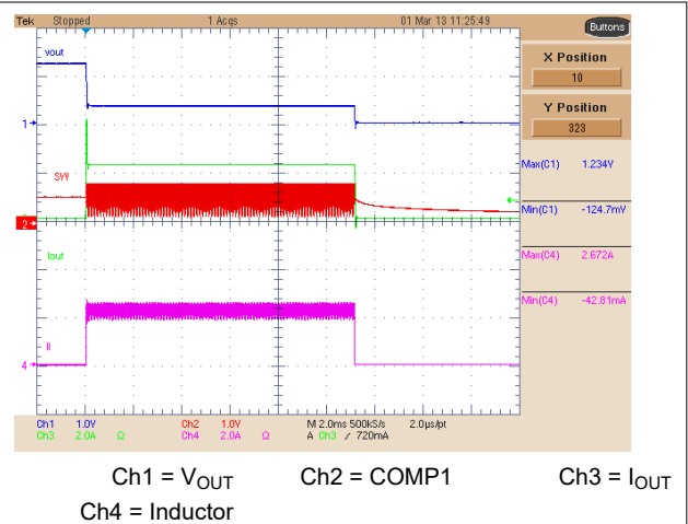
图 8-18. Buck 1 Current Limit Operation, Hiccup
