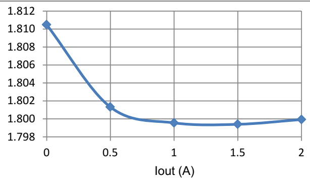
图 6-10. Load Regulation, 25^\circ\text{C} , 1% 100-PPM Resistor
