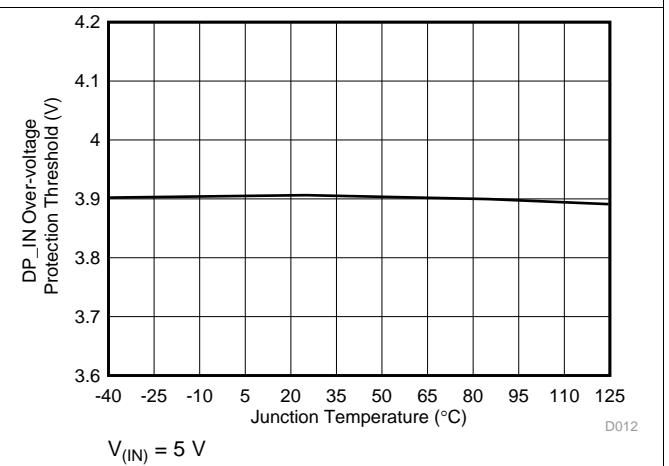
图 10. DP_IN Overvoltage Protection Threshold vs Temperature
