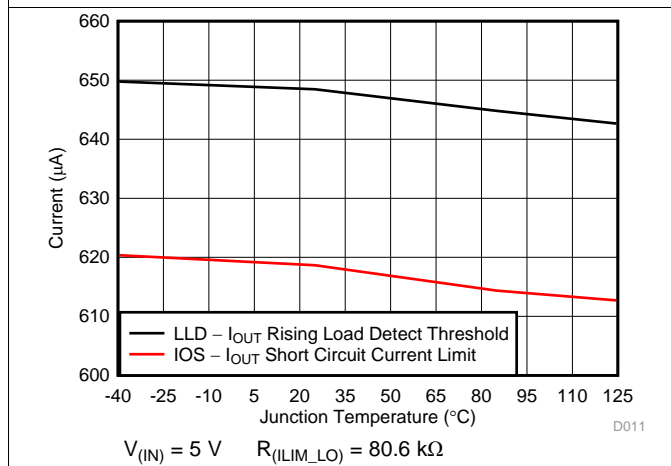
图 9. I_{(OUT)} Rising Load-Detect Threshold and OUT Short-Circuit Limit vs Temperature
