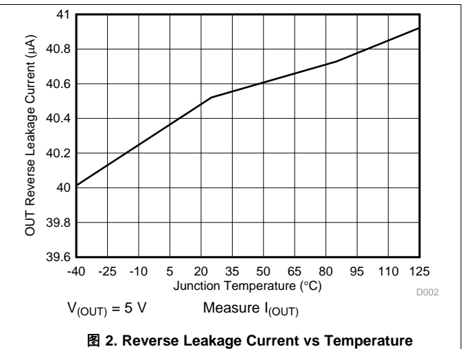
图 2. Reverse Leakage Current vs Temperature
