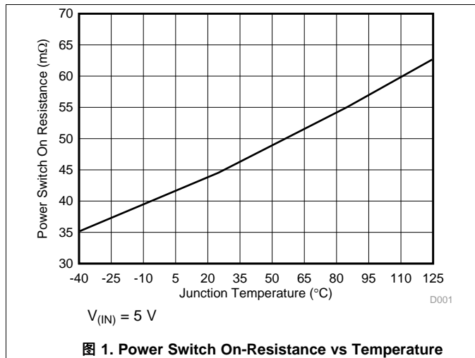
图 1. Power Switch On-Resistance vs Temperature
