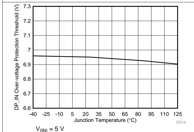
图 11. OUT Overvoltage Protection Threshold vs Temperature
