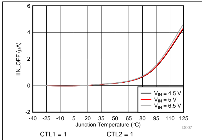
图 7. Disabled IN Supply Current vs Temperature
