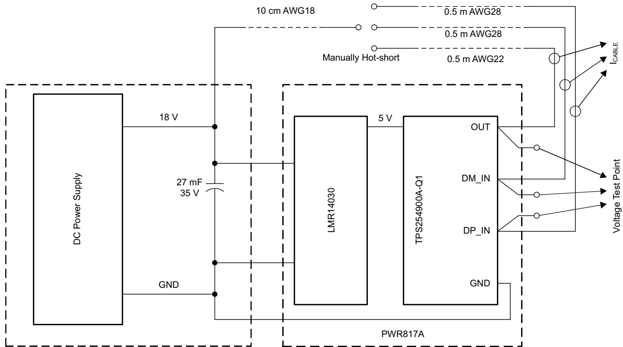
图 36. Short-to-Battery System Test Setup
