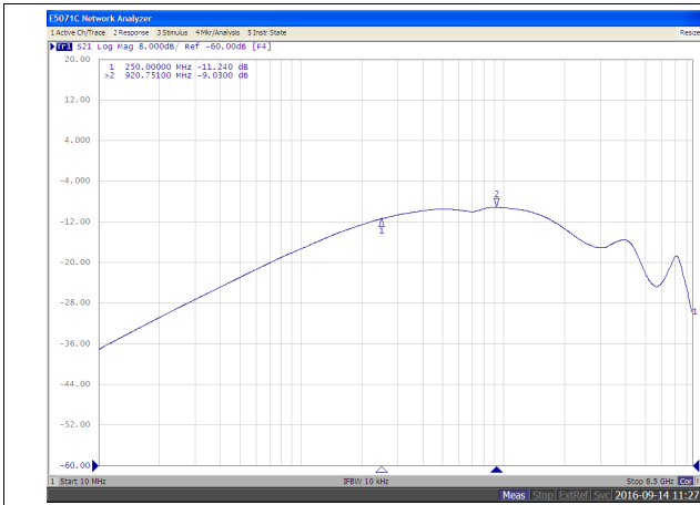
图 34. Off-State Data-Switch Isolation vs Frequency
