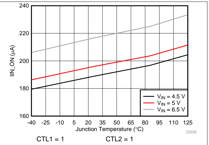
图 8. Enabled IN Supply Current – CDP (11) vs Temperature
